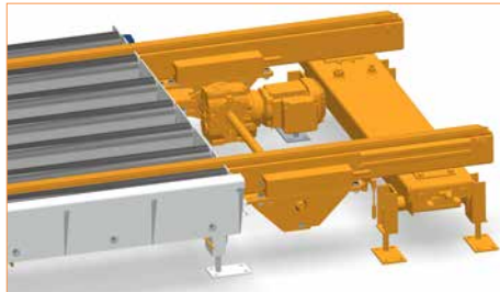
Transfer conveyor
